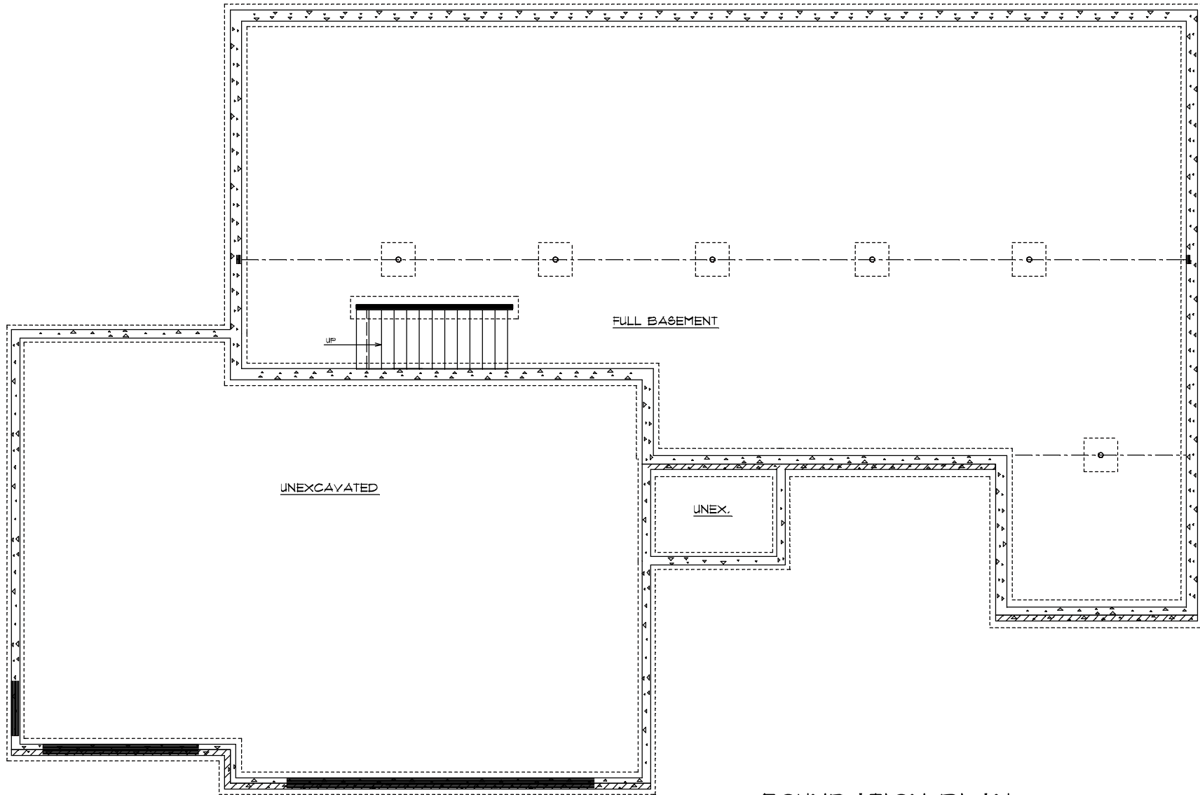
FOUNDATION PLAN
